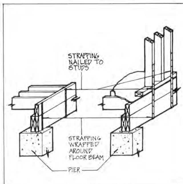
Figure 4.43. Metal Strapping
