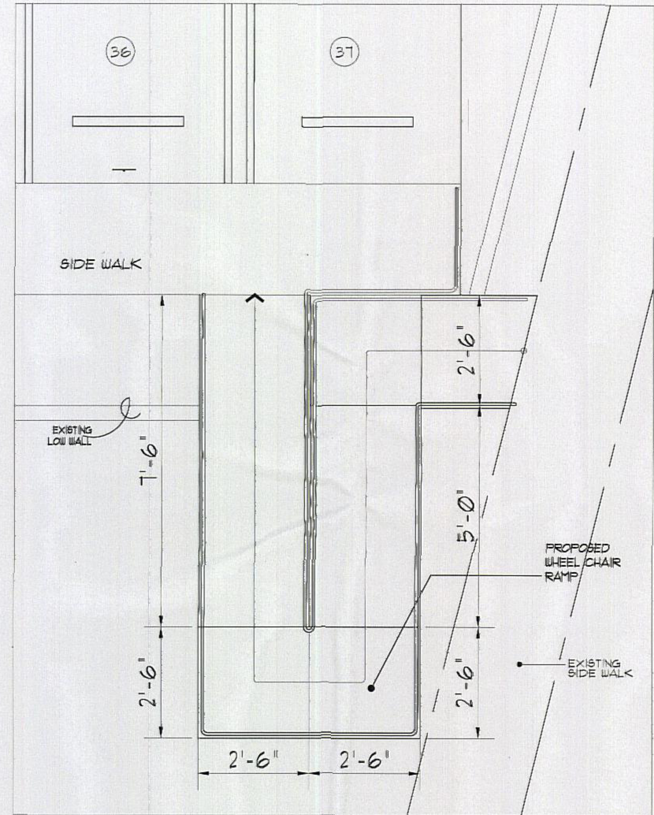
HANDICAP RAMP FLOOR PLAN SCALE: 1" = 1'-0"
