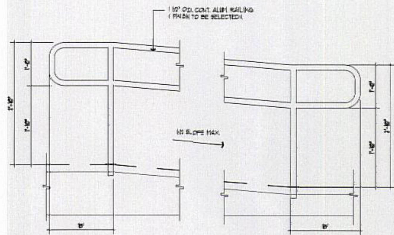
HANDICAP RAMP RAILINGS SCALE: 1" = 1'-0"
