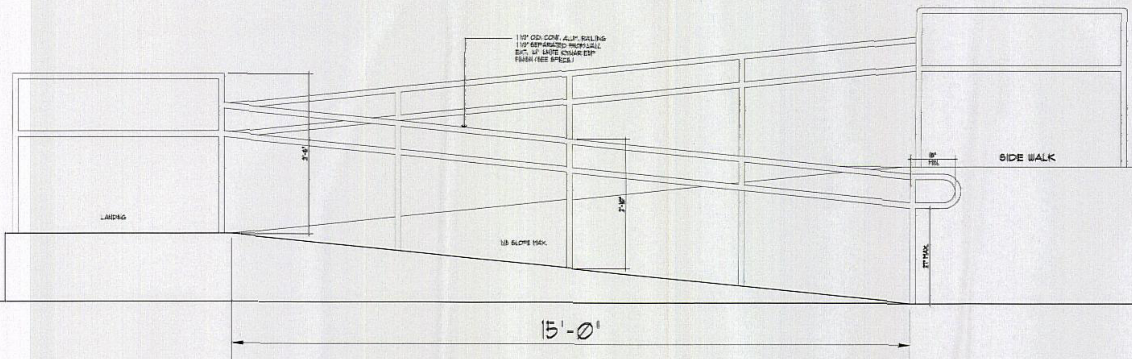
HANDICAP RAMP RAILINGS SCALE: 3/8" = 1'-0"
