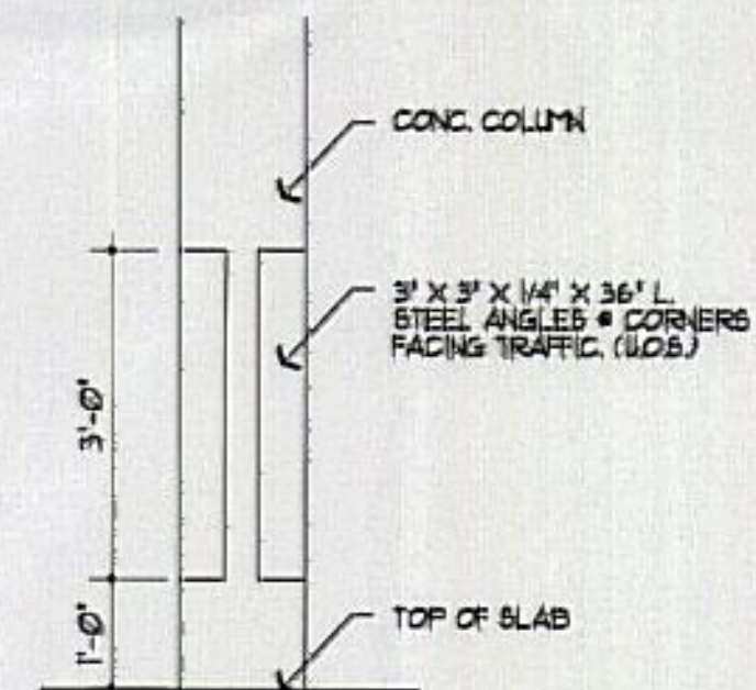
7 ADD'S COLUMN GUARD ELEVATION NTS.
