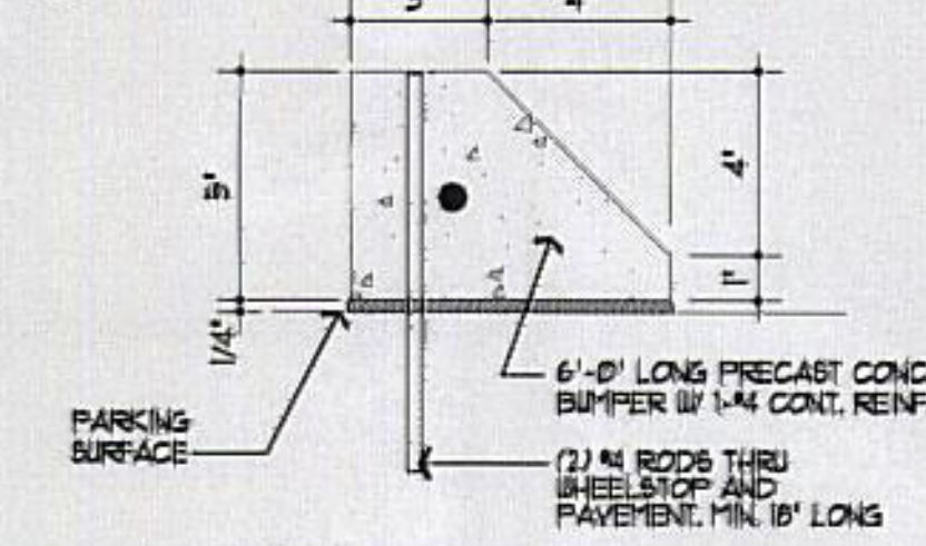
4 ADD'S TYP. WHEELSTOP @ ASPHALT NTS.
