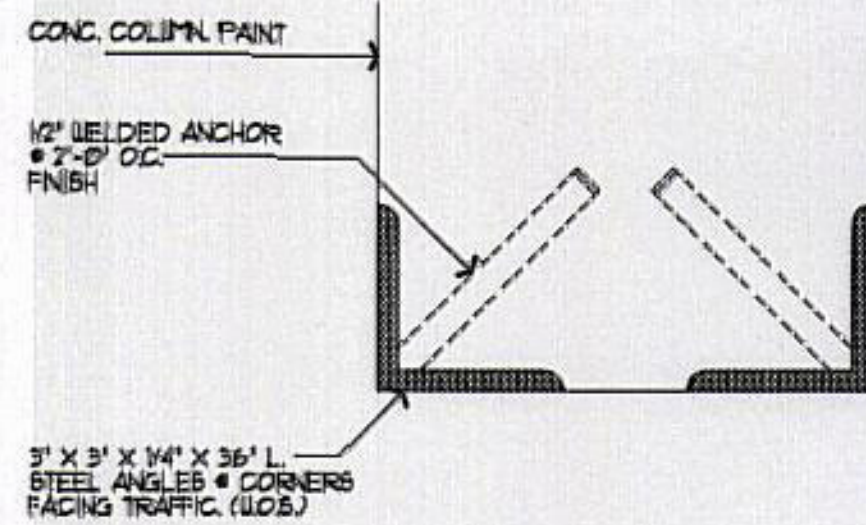
6 ADD'S COLUMN GUARD SECTION NTS.
