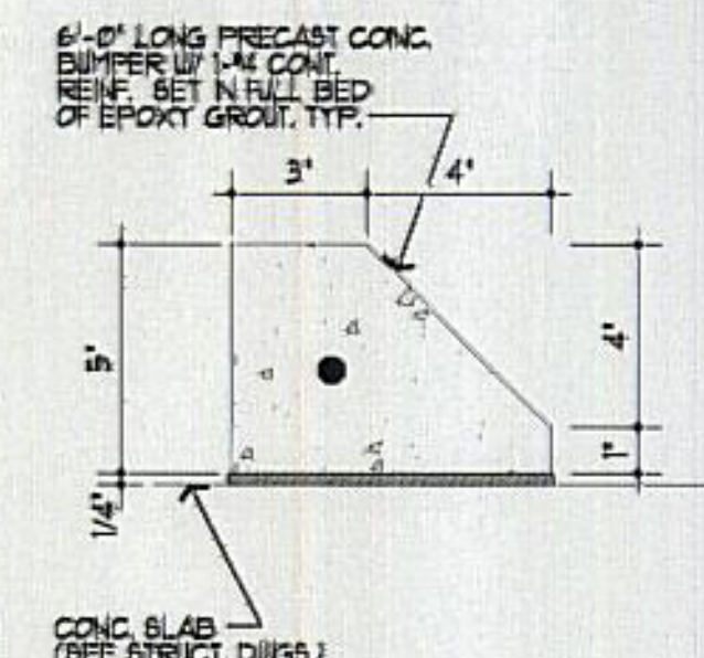
8 ADD'S TYP. WHEELSTOP @ SLAB NTS.
