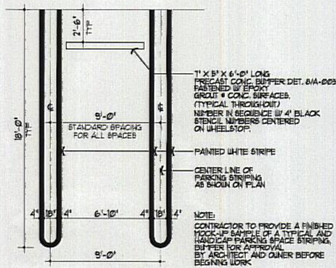
2 ADD'S TYP. PARKING STRIPING NTS.
