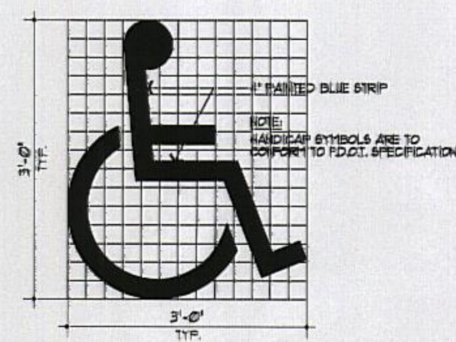
3 ADD'S TYP. HANDICAP SYMBOL NTS.
