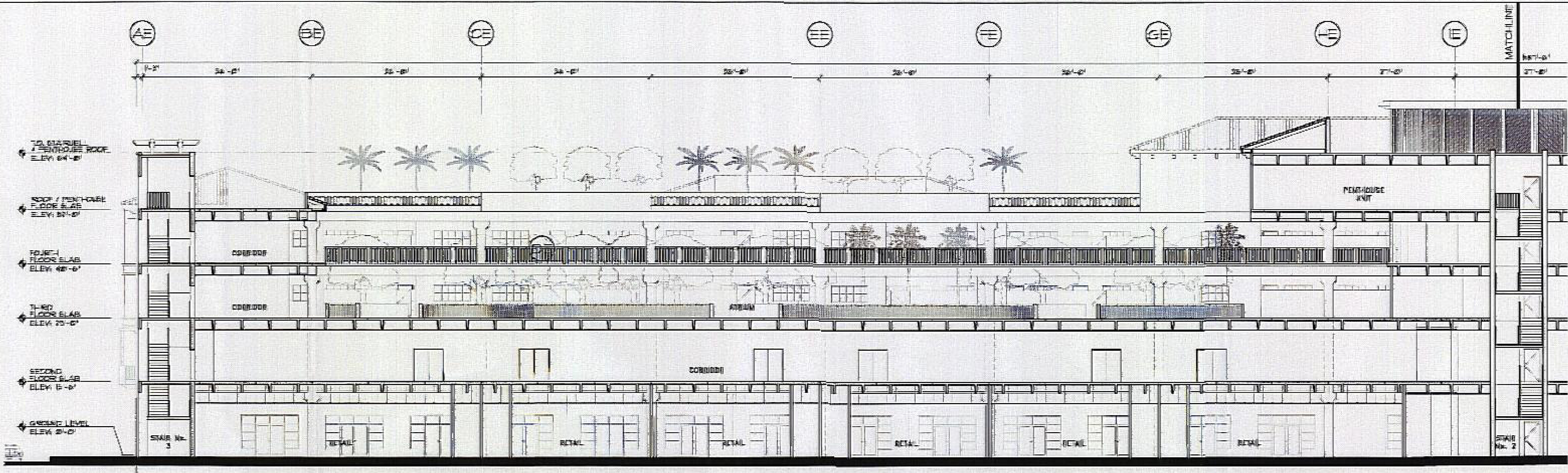
SECTION SCALE: 3/32" = 1'-0"
