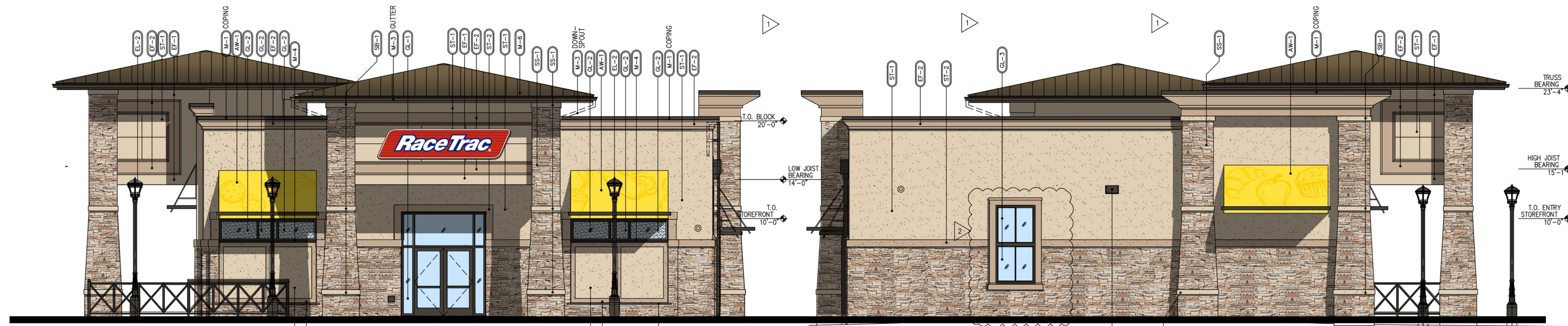
C RIGHT EXTERIOR ELEVATION
