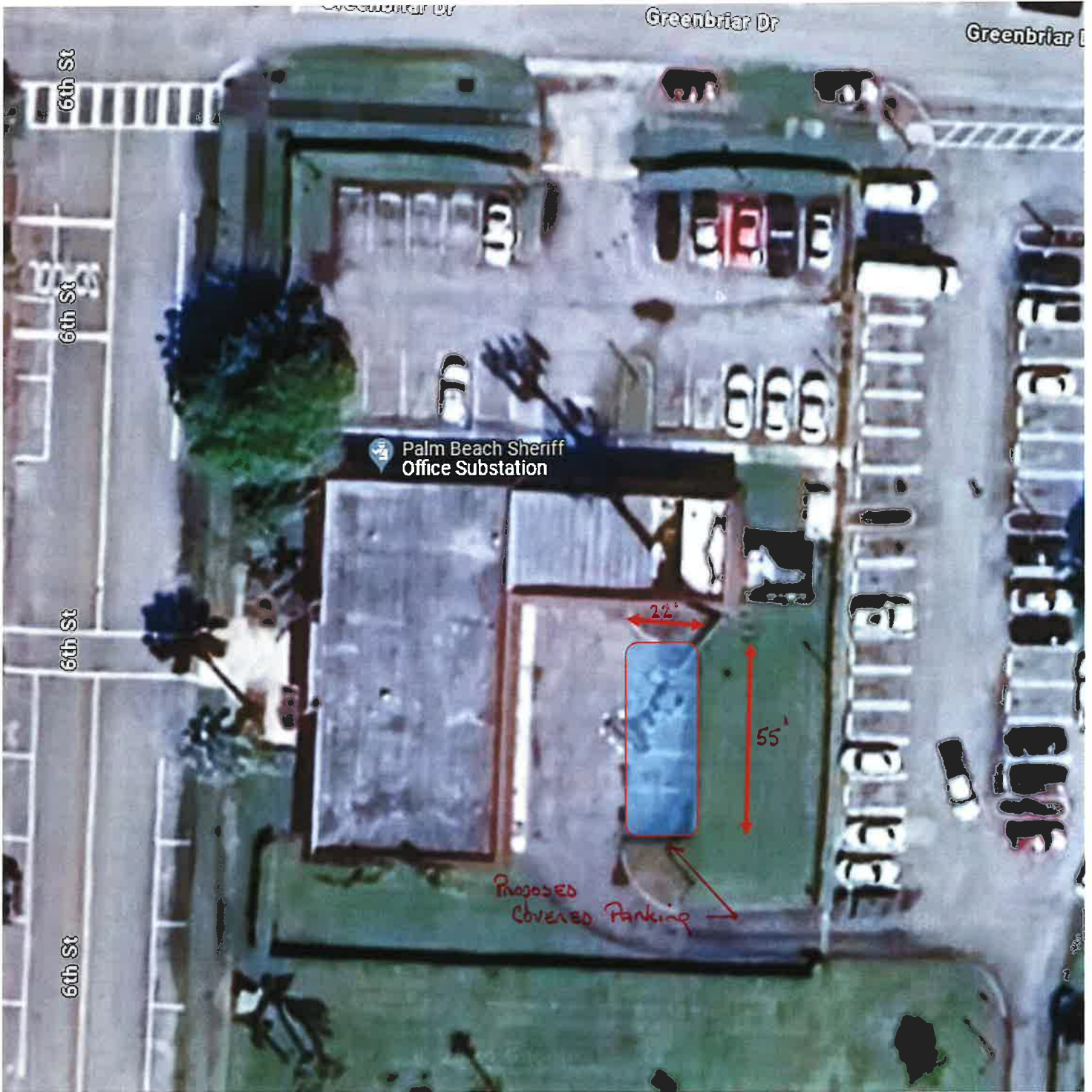
Open Air Covered Parking Carport Approximately 55' long x 22'-0" wide
